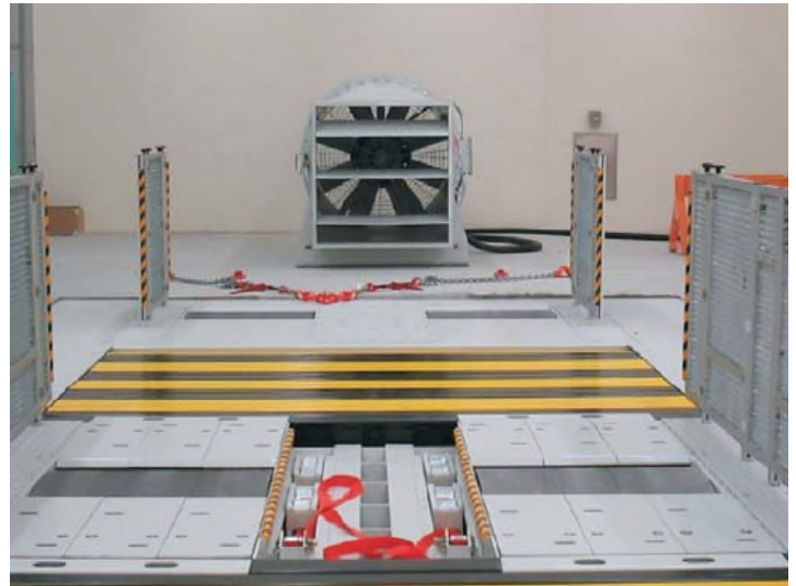
Movable test stand decking 'Pull Down' device ( option ) Automatic Wheel base adjustment ( Rear Axle )
