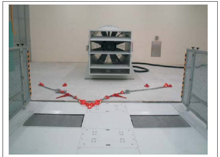
Fixed Roller Set ( Front Axle ) Vertical Wheel Guards Front Vehicle Fixing Device
